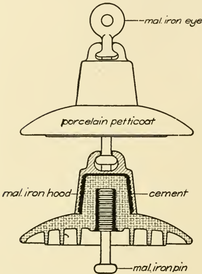
Fig. 179. Section of Suspension Insulator
